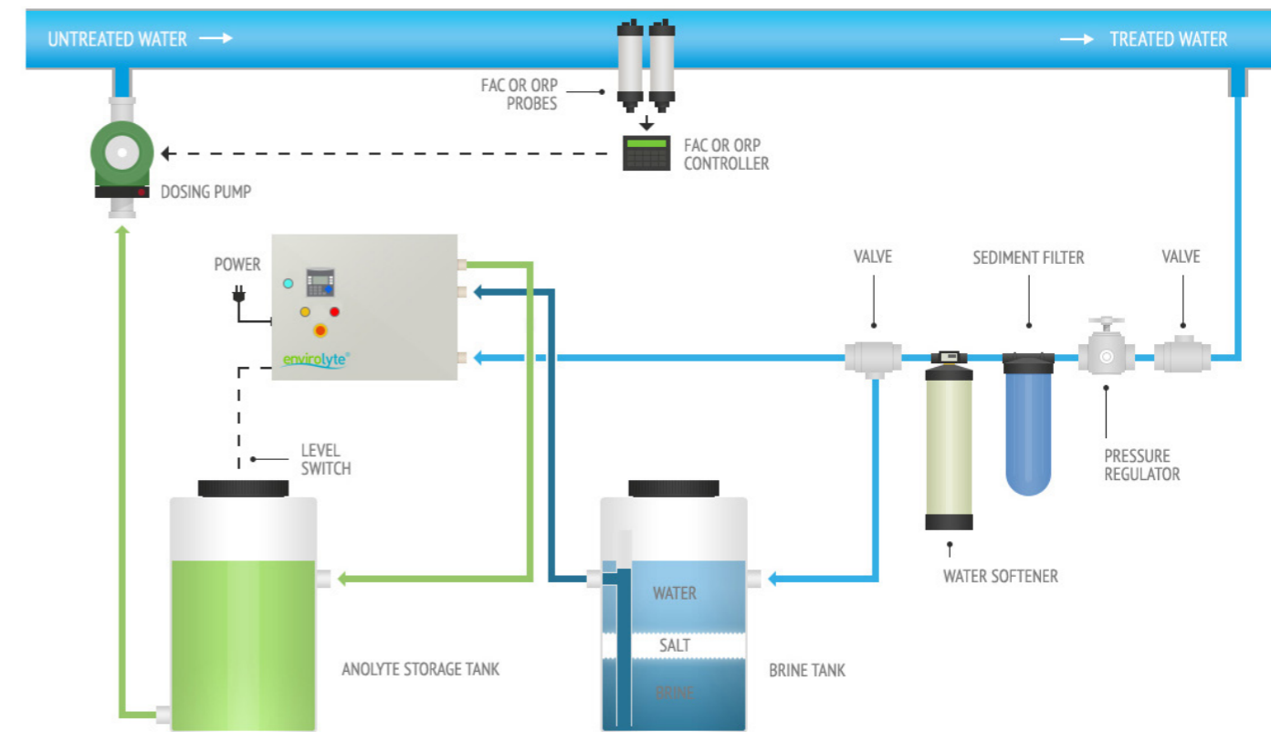
Typical layout of Enviolyte water disinfection system
